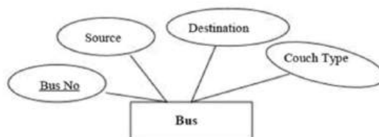
Bus: (Entity)
